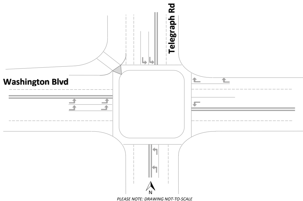
Figure 2: Intersection Diagram
